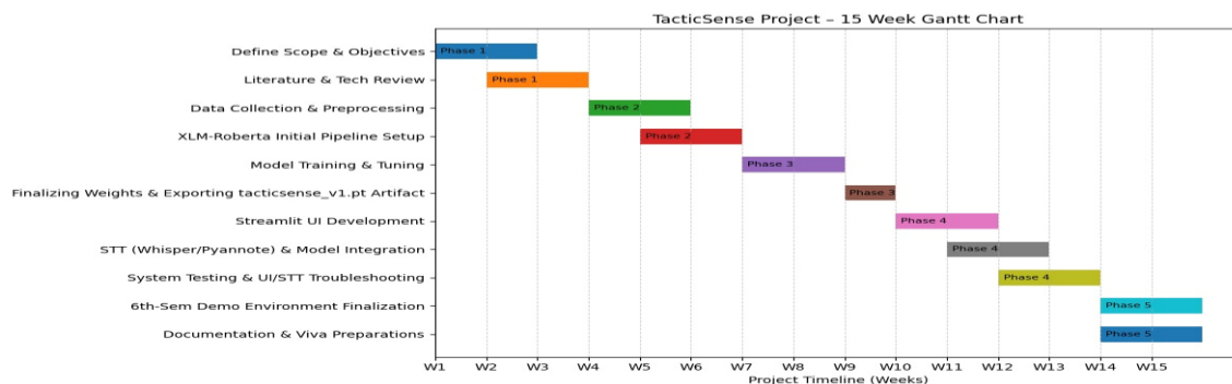
Fig 4.1-Gantt chart
