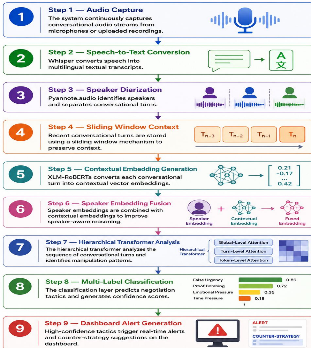
Fig 7.1 Implementation workflow
